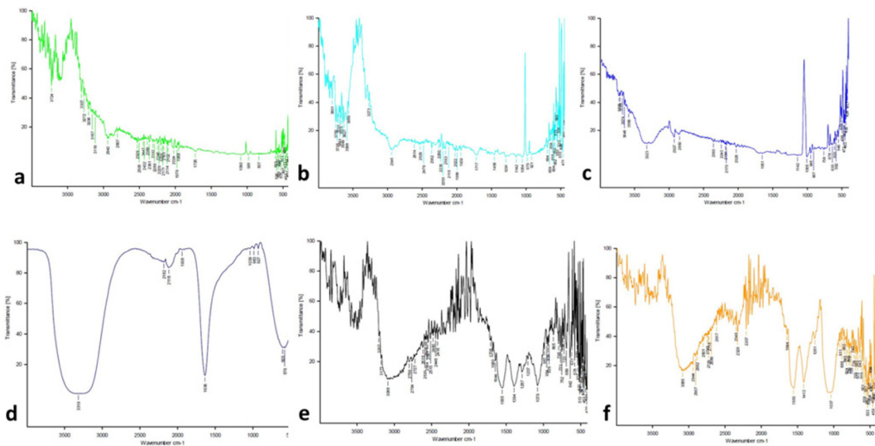
Fig. 1. FTIR spectra of (a) petroleum ether (b) benzene (c) chloroform (d) ethanolic (e) cold water and (f) hot water extracts of V. negundo leaves showing bands of different functional groups. Note the broad band at the range of 3600\text{--}3000\text{ cm}^{-1} in (d) spectra suggesting the presence of -OH group.
